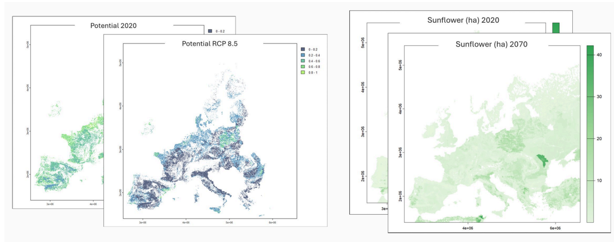
A representation of the spatial overlapping between pollination potential area (left) and demand area (right).
