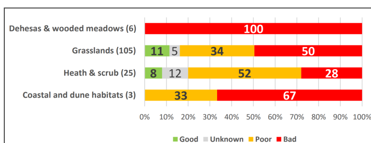
Conservation status of Annex I agricultural habitats in the EU in 2018. Source: EU (2023)(a) based on EEA data.
